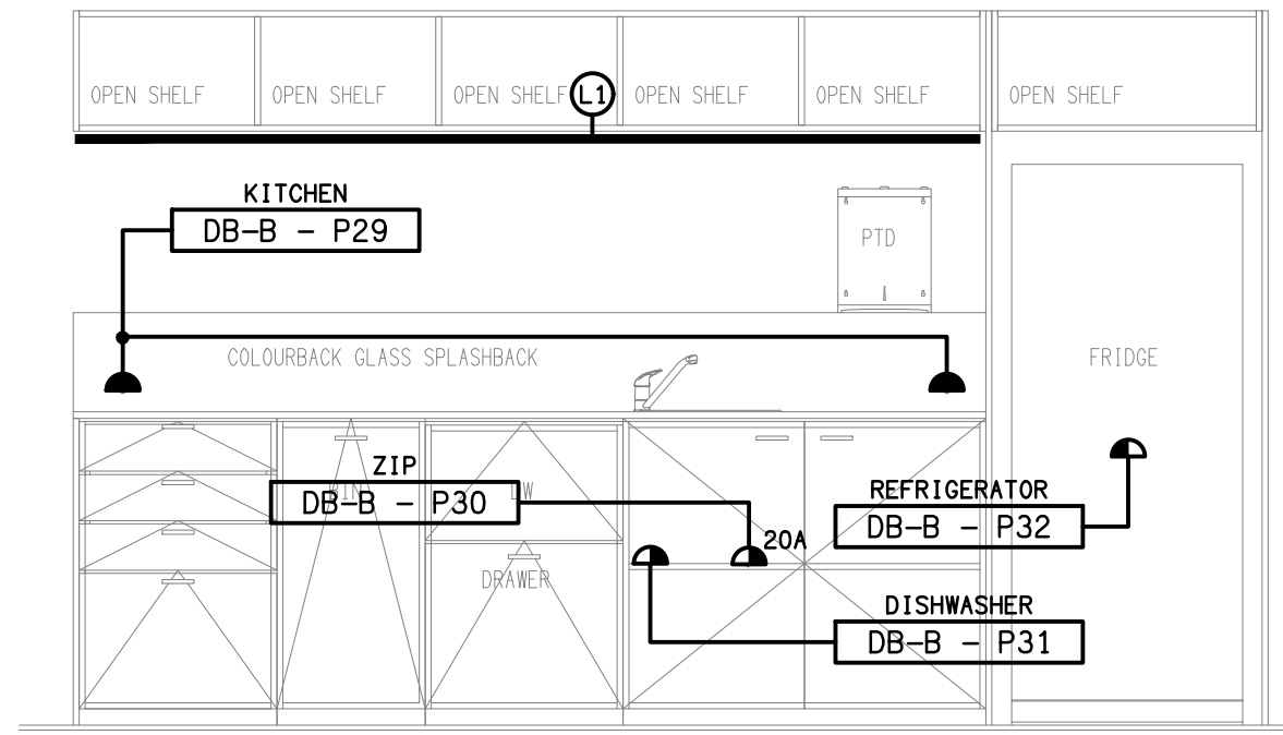
DETAIL C SHOWROOM CAFE KITCHENETTE SCALE 1: 25
