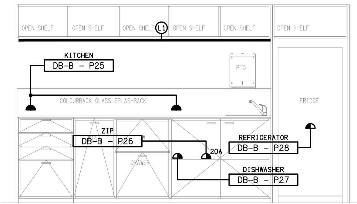
DETAIL B RECEPTION CAFE KITCHENETTE SCALE 1: 25
