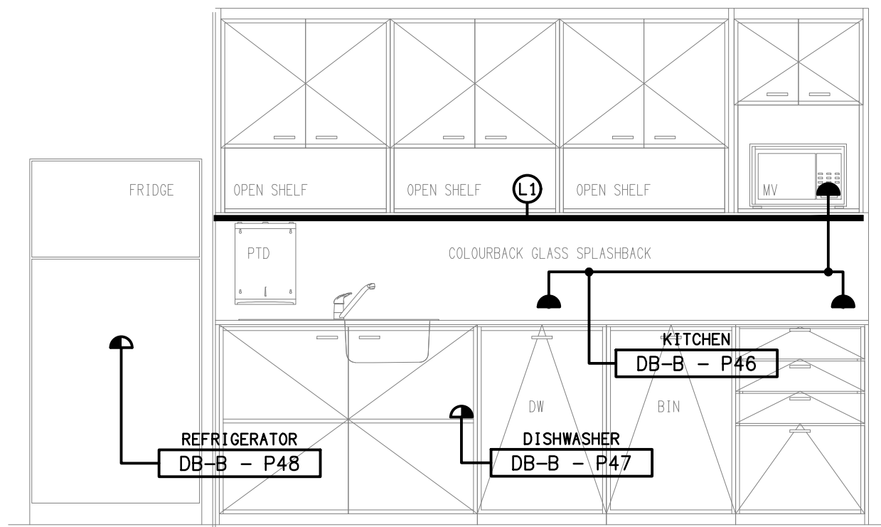
DETAIL D LUNCH ROOM 2 KITCHENETTE ELEVATION SCALE 1: 25
